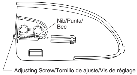
Figure 5 - Turning Adjusting Screw on Model 107624-01, -02
